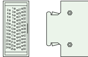
CN1 Connector (manufacturer: 3M) (Order code No.: FDA CON50P-3M)
