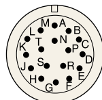
MS 3102A20-29P MS CONNECTOR
